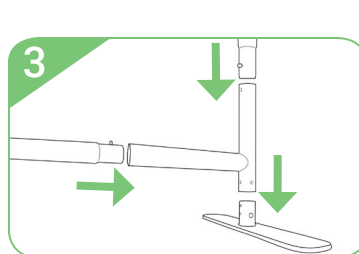
Attach corner tube onto feet. Then connect vertical and horizontal tubes to complete frame.
